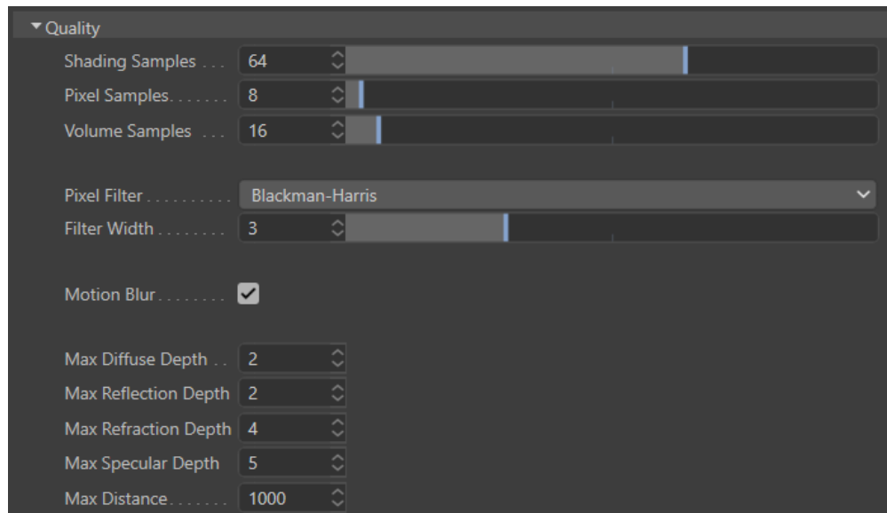
3Delight's Quality render settings.
