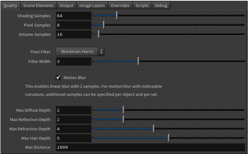
3Delight's Quality render settings.
